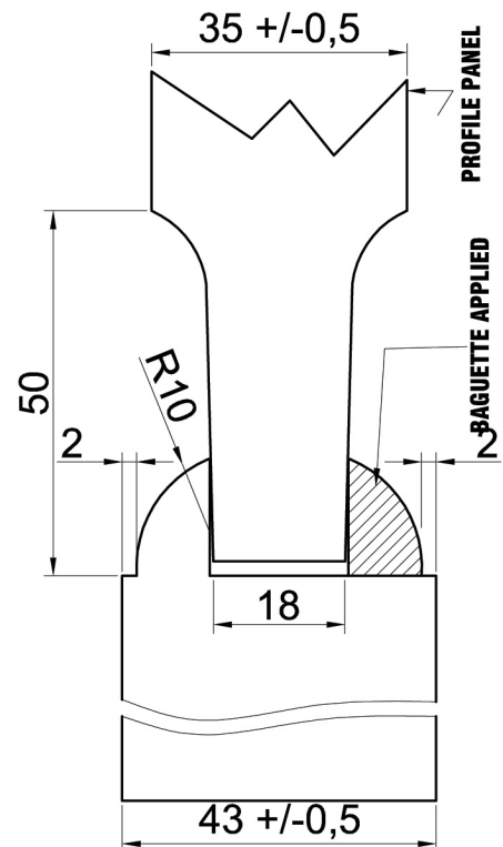
PROFILE OF THE STILE (UNIT IN mm) scale 1:1
