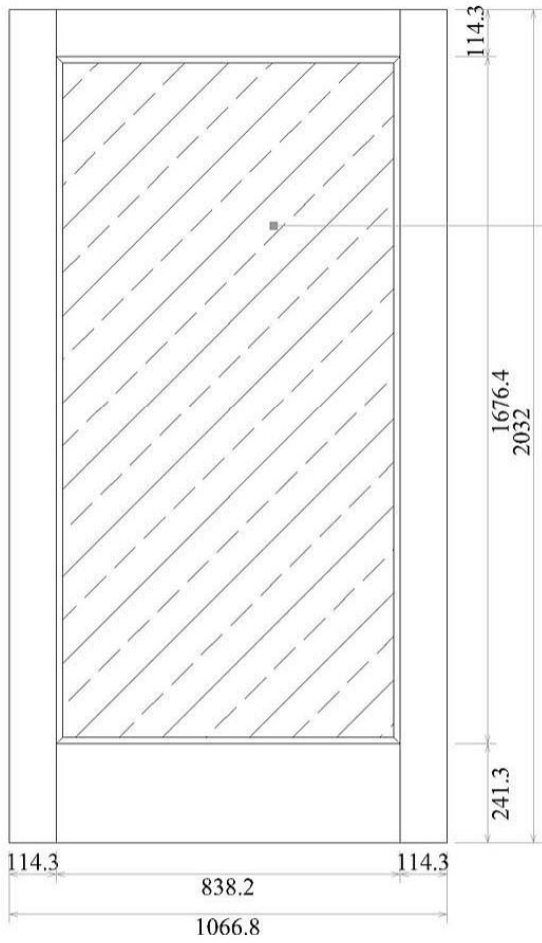
elevational view
